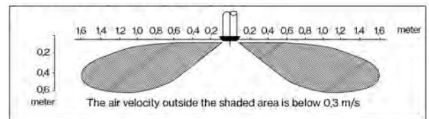
Distribution pattern at 70m³/h at 7 mm and 30 dB(A)
